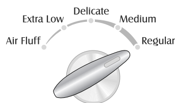
Infinite Temperature
